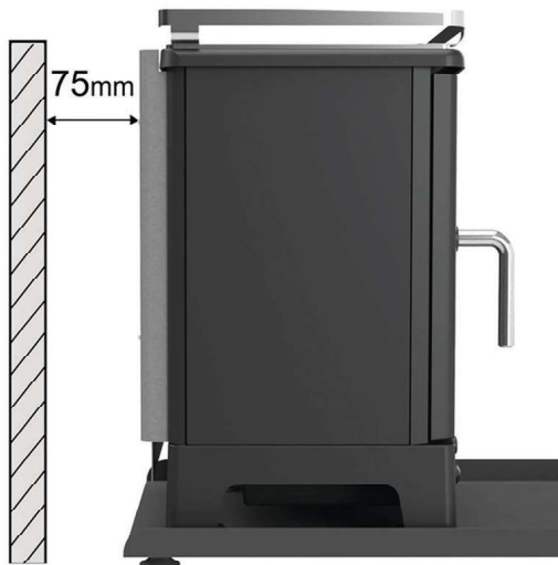
Distance to combustibles
